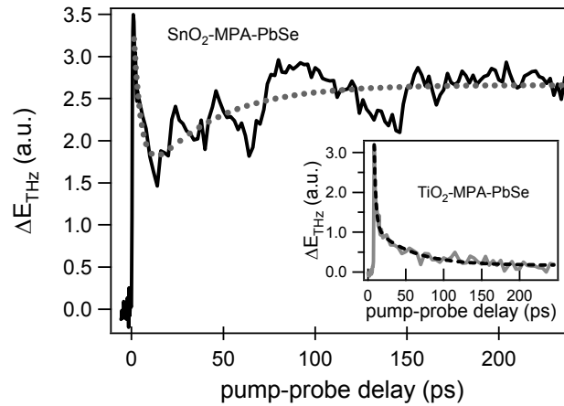
Figure 6.9. THz-TDS signal for the \text{SnO}_2 -MPA-PbSe sample (4.2 nm PbSe QDs), following photo-excitation with 800 nm pulses (500 \text{mJ}/\text{mm}^2 ). As for the \text{TiO}_2 -MPA-PbSe sample (inset), there is a quasi-instantaneous rise of the signal and a subsequent decay within tens of picoseconds. For the \text{SnO}_2 -MPA-PbSe sample, there is an additional long-lived ingrowth of the THz signal, which originates from injected electrons in \text{SnO}_2 . The dashed lines are fits to the data, yielding a timescale for electron injection of 40 \pm 10 ps.
