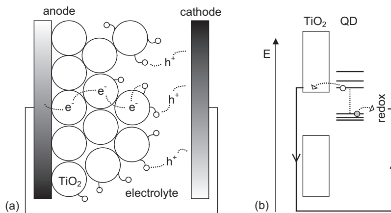
Figure 1.9 a) Schematic layout of a QD-sensitized solar cell (QDSSC), analogous to the Grätzel cell 36 , in which QDs are chemically linked to a mesoporous \text{TiO}_2 film. After excitation, electrons are injected from the excited QD into the \text{TiO}_2 conduction band and the remaining holes in the oxidized QD migrate towards the cathode via an electrolyte. b) Energetic band diagram of a QD sensitized solar cell.
