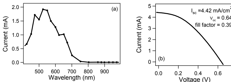
Figure 7.3 Photocurrent action spectrum (a) and I-V characteristics (b) of a N719-sensitized solar cell.
