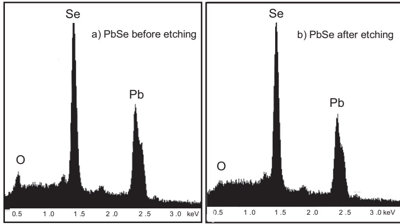
Figure 5.2. EDX spectra of the PbSe film (a) before etching and (b) after etching with a 10% HCl solution
