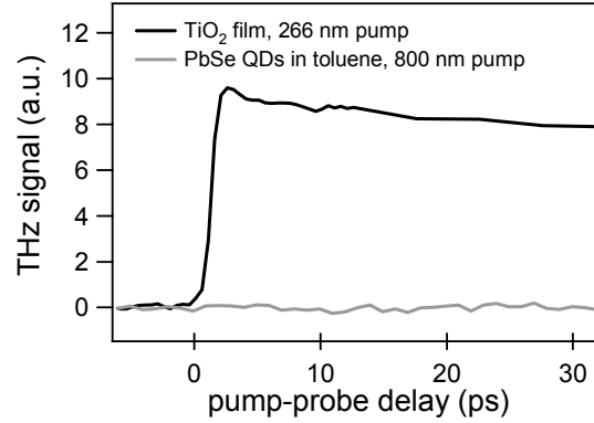
Figure 6.5 Comparison of the imaginary THz response for isolated PbSe QDs in toluene (grey line) and the real THz response for a directly excited unloaded \text{TiO}_2 film (black line). The unloaded film was directly excited with 266 nm pulses and the PbSe QDs sample was excited with comparable 800 nm fluences. Clearly, the (imaginary) THz signal arising from isolated QDs is negligible compared to the (real) signal from carriers in the \text{TiO}_2 film.
