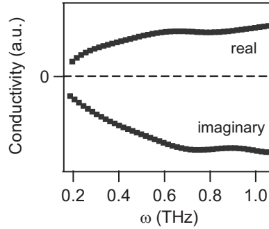
Figure 6.7 Complex conductivity of the \text{TiO}_2 -MPA-PbSe film, measured 30 ps after photo-excitation with 800 nm light. The shape of the conductivity is characteristic for the presence of free carriers in nanostructured semiconducting materials 24,32 .
