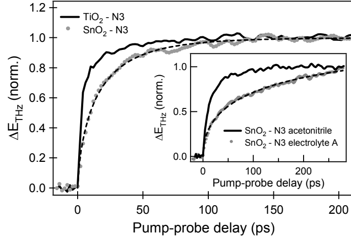
Figure 7.8 THz modulation for N3-sensitized SnO 2 (grey dots) and TiO 2 (black lines) following excitation with 590 nm pulses. In contrast with injection into TiO 2 , electron injection into SnO 2 is not bi-phasic and can be fit with a stretched exponential ingrowth. The dynamics of the THz data are attributed to injection from the 3 MLCT state, as explained in the text. The inset shows a comparison of injection dynamics into SnO 2 in acetonitrile and electrolyte A.
