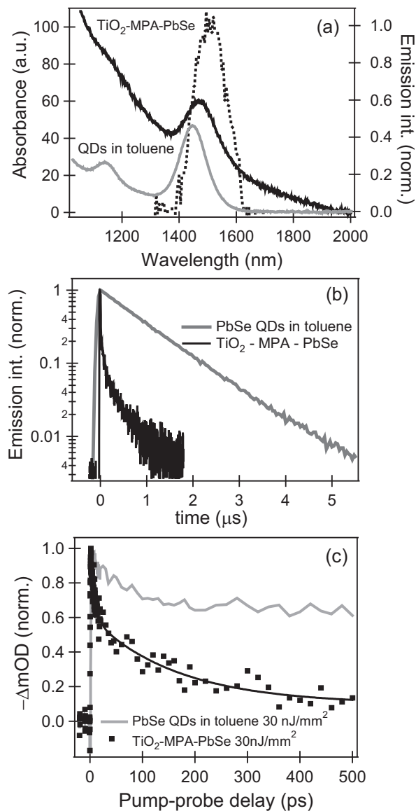
Figure 6.4 a). Absorption spectrum of 4.2 nm PbSe QDs in toluene (grey solid line) and a \text{TiO}_2 -MPA-PbSe sample (black solid line). The dashed line is the luminescence spectrum of the \text{TiO}_2 -MPA-PbSe sample. b). Decay of the luminescence for the same PbSe QDs in toluene (grey line), which can be fitted with an exponential decay using a time constant of \sim 1.0 \mu\text{s} . The black line corresponds to the luminescence decay of the \text{TiO}_2 -MPA-PbSe sample. c). Normalized decay dynamics of TA measurements for 4.2 nm PbSe QDs in toluene (grey solid line) and for the \text{TiO}_2 -MPA-PbSe sample (black dots). For both experiments, an 800 nm excitation fluence of 30 \text{ nJ/mm}^2 was used and the photo-induced bleaching of the 1S transition was probed using 1500 nm pulses.
