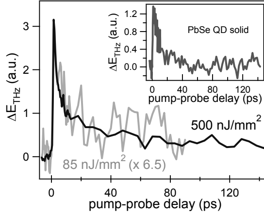
Figure 6.6 THz-TDS signals for the \text{TiO}_2 -MPA-PbSe sample (4.2 nm PbSe QDs), following photo-excitation with 800 nm pulses. The similarity between results at different fluences (black trace: 500 \text{ nJ/mm}^2 and grey trace: 85 \text{ nJ/mm}^2 ), apart from a scaling factor, reveals that effects due to multi-photon absorption are negligible. The real conductivity represented by the THz signals does not originate from free carriers in \text{TiO}_2 but is likely due to mobile carriers in QD clusters at the \text{TiO}_2 surface, as explained in the text. The inset shows the THz signal of a PbSe QD solid on fused silica for an 800 nm excitation fluence of 500 \text{ nJ/mm}^2 .
